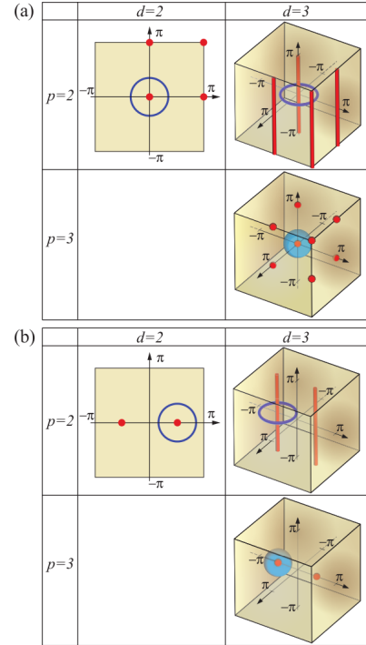
FIG. 11 (Color online) The classification of stable Fermi surfaces depends on how the Fermi surfaces transform under non-spatial antiunitary symmetries, and hence their location in the Brillouin zone. Here, d denotes the spatial dimension (the dimension of the Brillouin zone) and p is the codimension of the Fermi surface. The blue circles/spheres represent the contour on which the topological invariant is defined. (a) Each Fermi surface (red point/line) is left invariant under non-spatial symmetries. (b) Different Fermi surfaces are pairwise related by the non-spatial symmetries which map \mathbf{k} \leftrightarrow -\mathbf{k} . Adapted from (Chiu and Schnyder, 2014).
