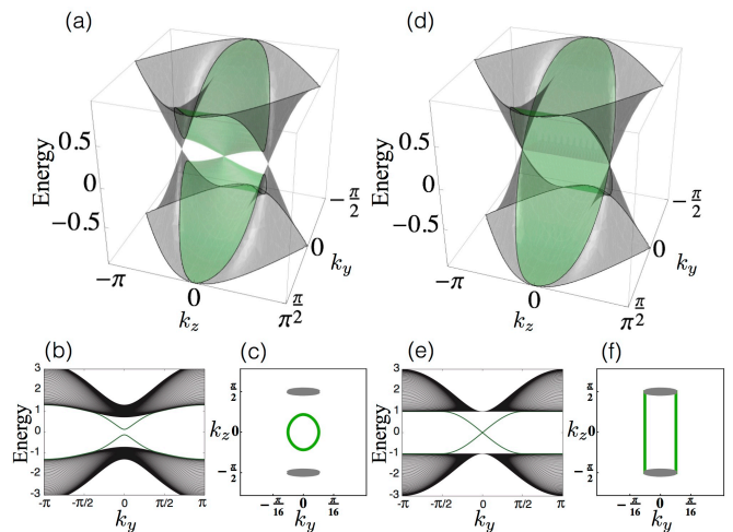
FIG. 13 Surface spectrum of the time-reversal symmetric (i.e., without Zeeman term) Dirac semimetal (5.4) for the (100) face. The surface and bulk states are colored in green and gray, respectively. Panels (a)-(c) and (d)-(f) show the surface spectrum in the presence and absence of the surface perturbation +g \sin k_z \tau_1 s_3 , respectively, which breaks reflection and chiral symmetry. Panels (b) and (e) show the surface bands as a function of surface momentum k_y with fixed k_z = \pi/4 and k_z = 0 , respectively. Panels (c) and (f) show the bulk and surface states for a fixed energy \varepsilon = 0.1 . The surface Dirac cone of panel (a) is protected by a \mathbb{Z}_2 invariant, while the surface Fermi arc of panel (d) is protected by the mirror winding number \nu^+ (see Sec. V.B.2.a).
