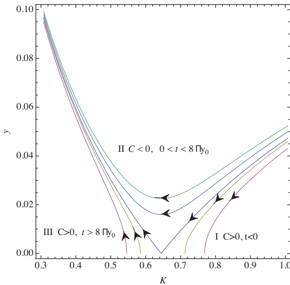
FIGURE 2. Renormalization group flows from equation (1) for the 2D planar rotor model. Note that for T \leq T_c , y(\infty) = 0 and K^{-1}(\infty) = \pi/2 .
