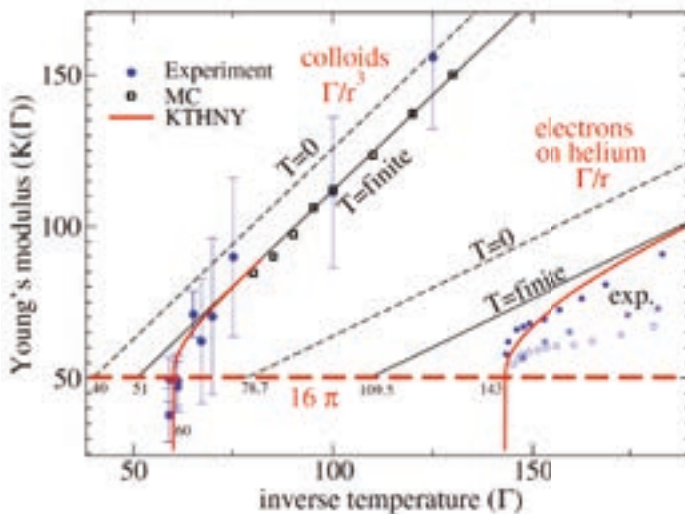
FIGURE 5. Young’s modulus K_R(T) as a function of the effective inverse temperature \Gamma . The solid line is the dislocation theory prediction of Halperin and Nelson and the symbols are the experimental points. Reprinted from Fig. (2) of J. Phys.: Condens. Matter 17 (2005) S3579-S3586 doi: 10.1088/0953-8984/17/45/051 with permission. Copyright 2005 IOP.
