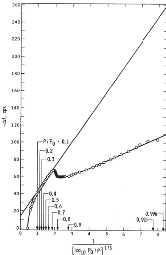
FIGURE 1. The horizontal axis is a measure of the total areal mass density of the adsorbed film and the vertical axis is -\Delta f , a measure of the adsorbed mass which decouples from the oscillating substrate. Reprinted from M. Chester, L. C. Yang and J. B. Stephens, Phys. Rev. Lett. 31 211 (1972) with permission. Copyright American Physical Society.
