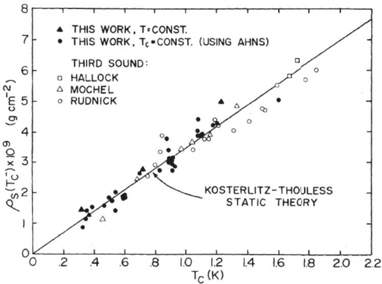
FIGURE 3. Results of third sound and torsional oscillator experiments for the superfluid density discontinuity \rho_s(T_c^-) as a function of temperature. The solid line is the theoretical prediction for the static theory. Reprinted from D J Bishop and J D Reppy, Phys Rev Lett 40 1727 (1978) with permission. Copyright American Physical Society.
