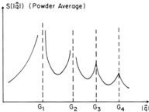
FIGURE 4. A schematic sketch of the structure function S(\mathbf{q}) of a 2D crystal. For T \leq T_m , peaks for small \mathbf{G} diverge as |\mathbf{q} - \mathbf{G}|^{-2+\eta_G} but for larger \mathbf{G} are finite cusps. For T > T_m , all peaks are finite with maximum height \sim \xi_+(T)^{2-\eta_G} . Reprinted from [34] with permission. Copyright 2002 Cambridge University Press.
